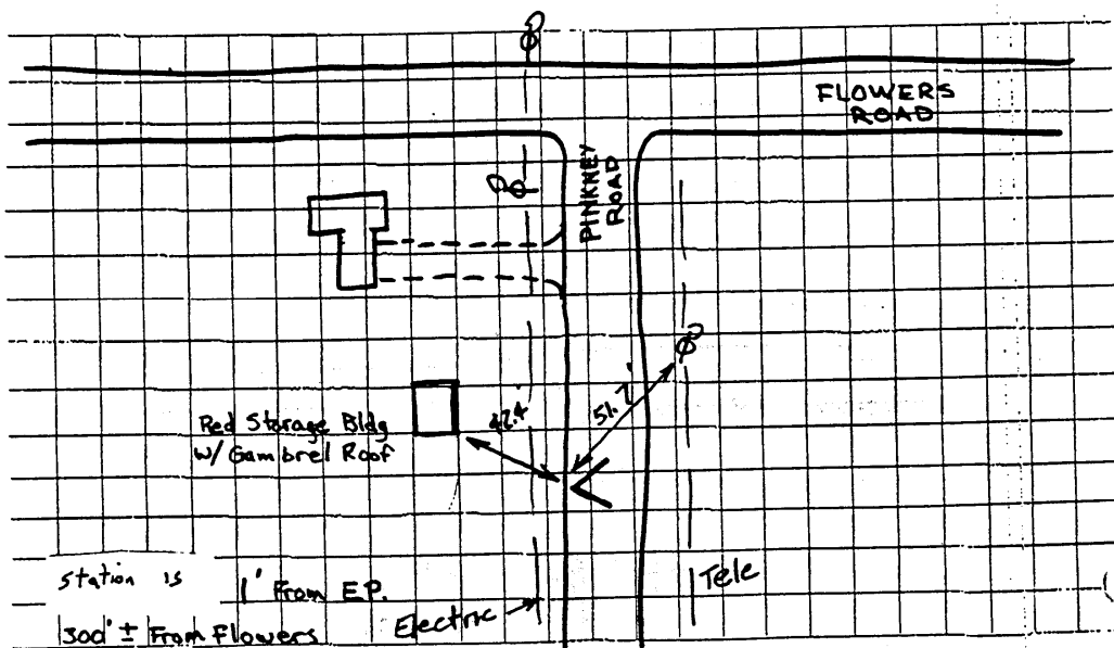
STATION SKETCH
