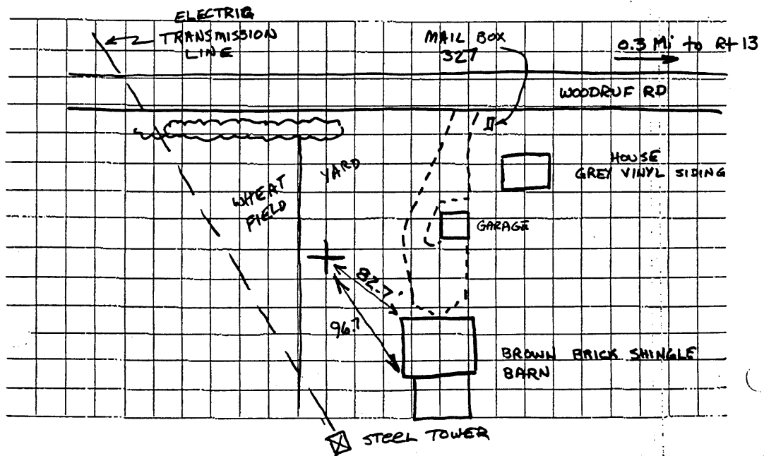
STATION SKETCH
