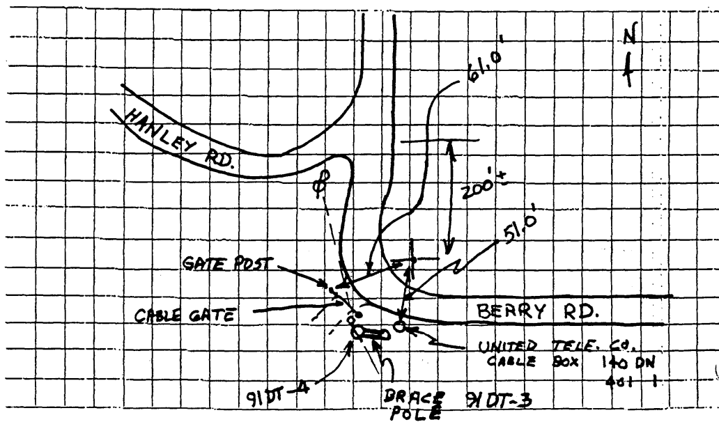
STATION SKETCH
