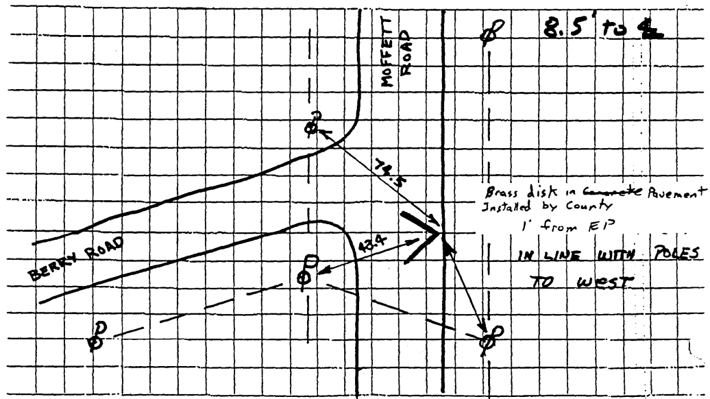
20' 1/8" STATION SKETCH
