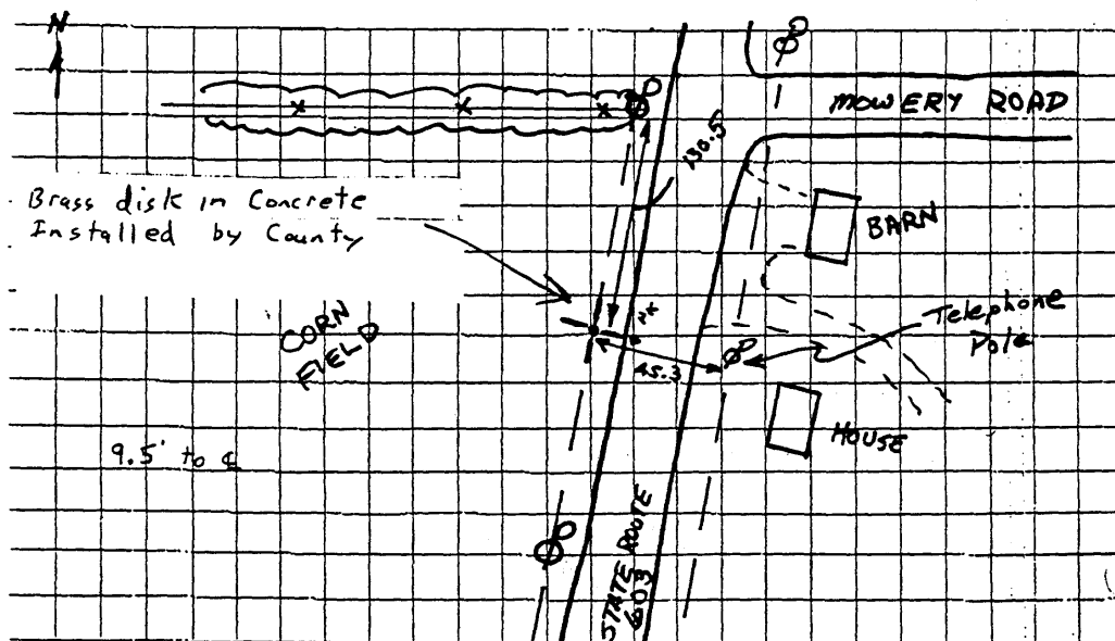
STATION SKETCH
