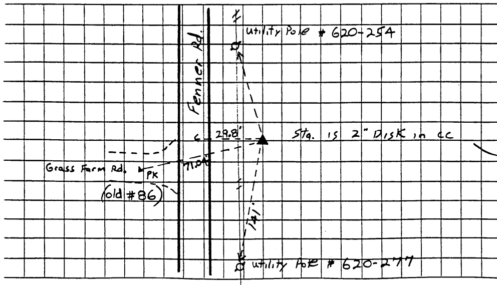
STATION SKETCH
